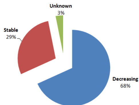
Figure 6: Local population trend of indigenous fishes of the Brahmaputra River
