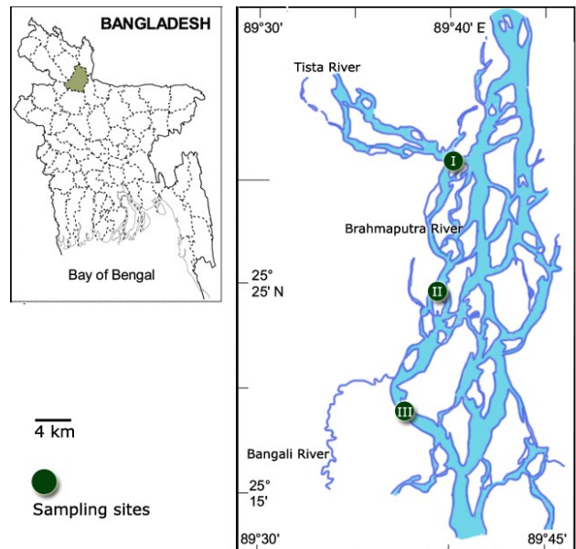
Figure 1: Map of the Brahmaputra River in Gaibandha district of Bangladesh showing the sampling sites; (I) Chandipur, (II) Mollarchar and (III) Fulchari Ghat
